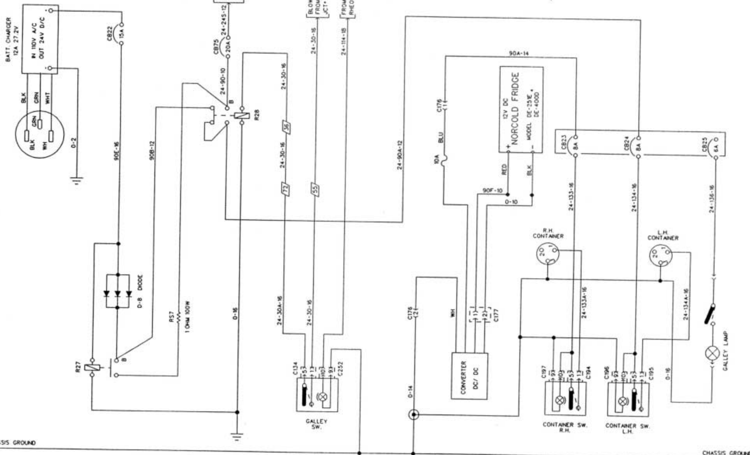
GALLEY "MINI-CHEF" NORCOLD REFRIGERATOR
